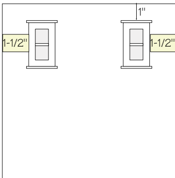
S1 Shown: Window # 1 Can Use # 4
