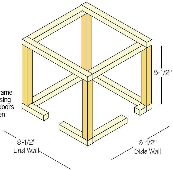
Build this frame if you are using Garden Town Doors and Windows
