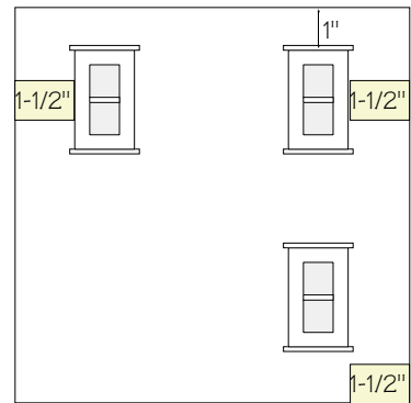
S2 Shown: Window # 1 Can Use # 4
