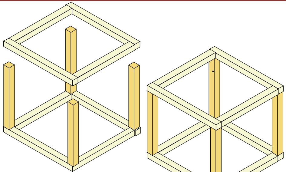
Build this frame if you are using Garden Town Doors and Windows
